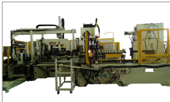
3-roll rolling/sizing/plasma welding Machine 3輪捲圓/整圓/等離子焊接機
