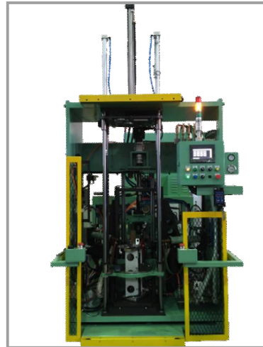
Press fit/2 spot welding for inner plate, and pipe expanding MC 插入點焊鉚合機
